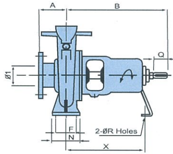
Dimension - Flange (JIS 10K RF)
