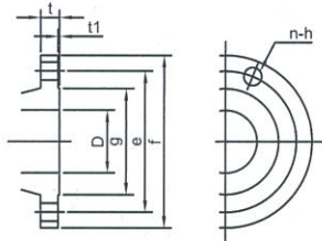
Dimension - Pump (JIS 10K RF)
