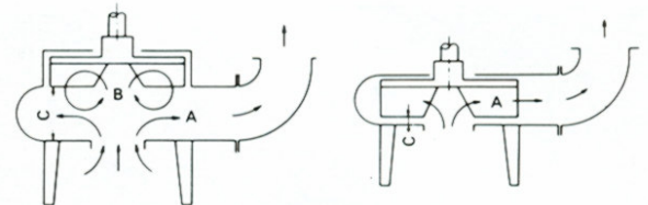
Conventional non-clog pump
